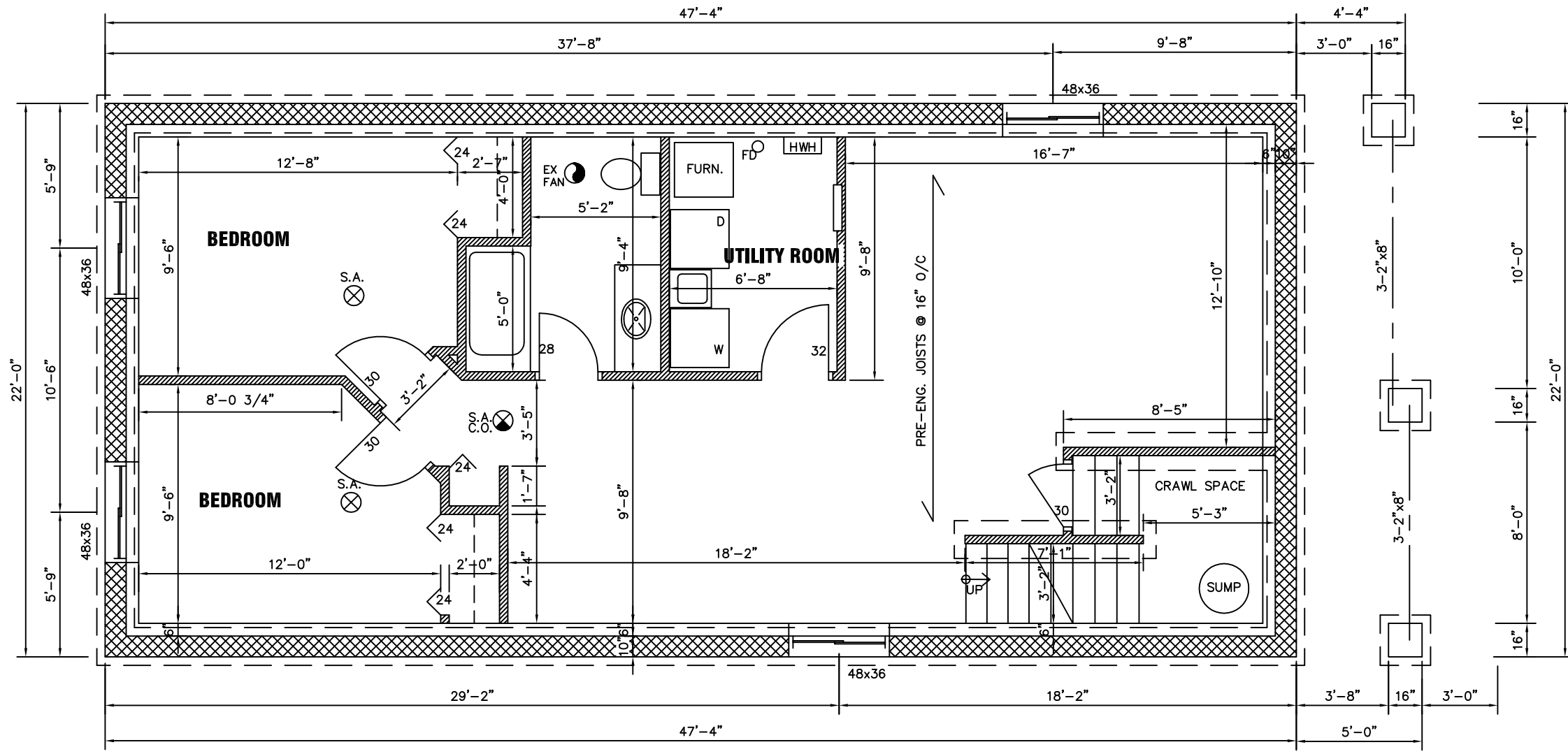
BASEMENT PLAN -2 BEDROOM
